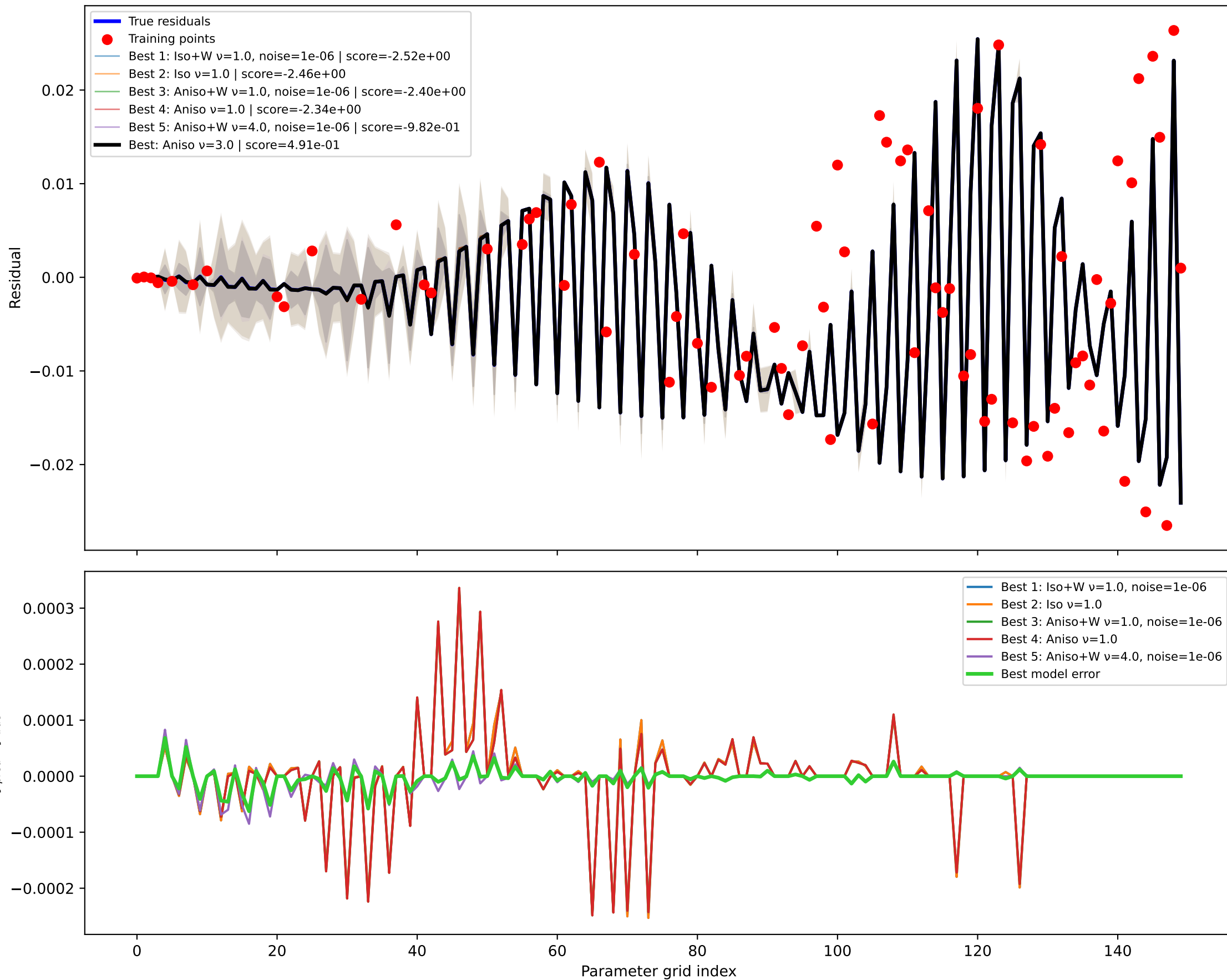
GPR kernel comparison node=26 RMSE=1.608e-05, train RMSE=2.697e-11
